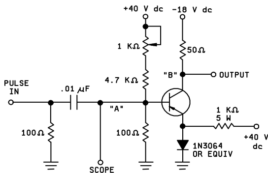
MIL-PRF-19500/177F FIG 2. Nonsaturated switching time test circuit.
