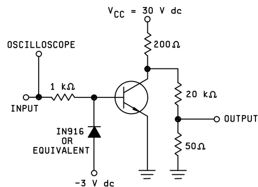
FIG 18. Saturated turn-off switching time test circuit.
